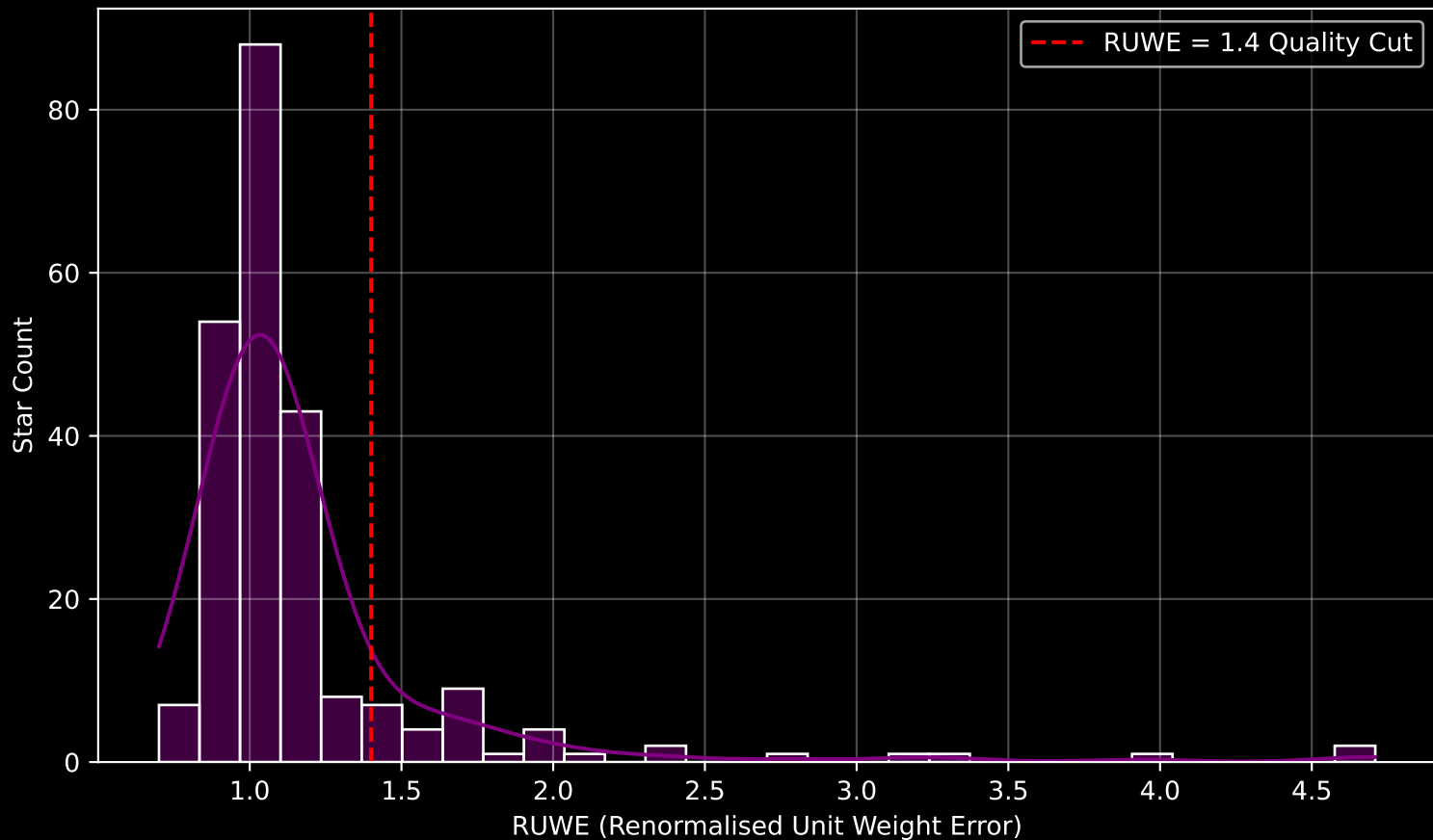
GALAH DR4 Field [7224] RUWE Distribution (n= 234)
