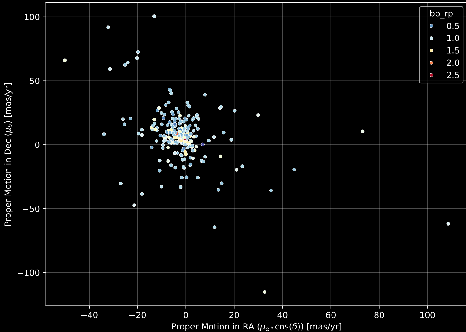
GALAH DR4 Field: [7224] Proper Motion Diagram (n= 248)
