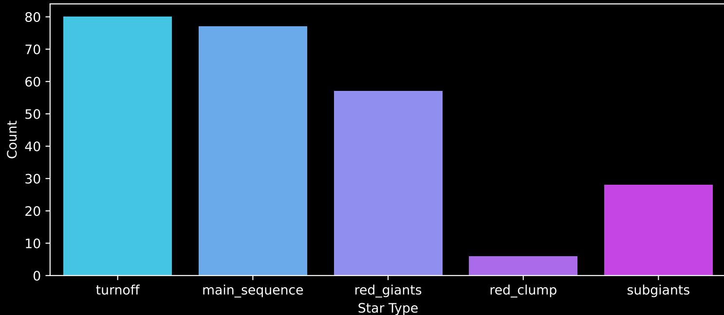
GALAH DR4 Field: [7224] Count plot of Star Type
