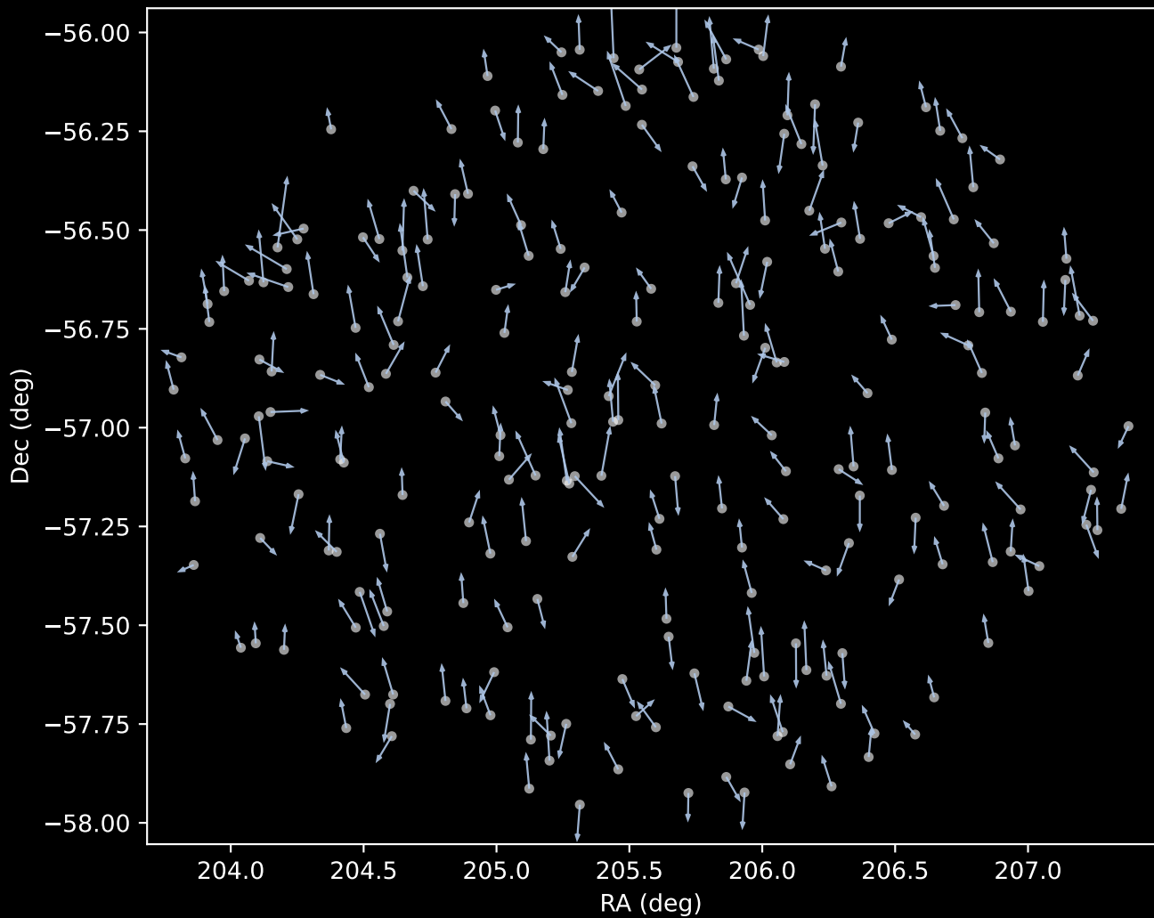
GALAH DR4 Cluster 1 Proper Motion Vectors (n=236)
